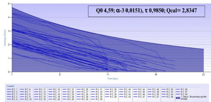
Fig. 3. MRC using the Deput-Boussinesq aquifer storage model for the Wae Ruhu Watershed.
