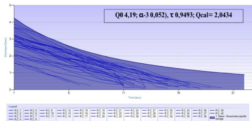
Fig. 6. MRC using Deput-Boussinesq aquifer storage model for the Wae Tomu Watershed.
