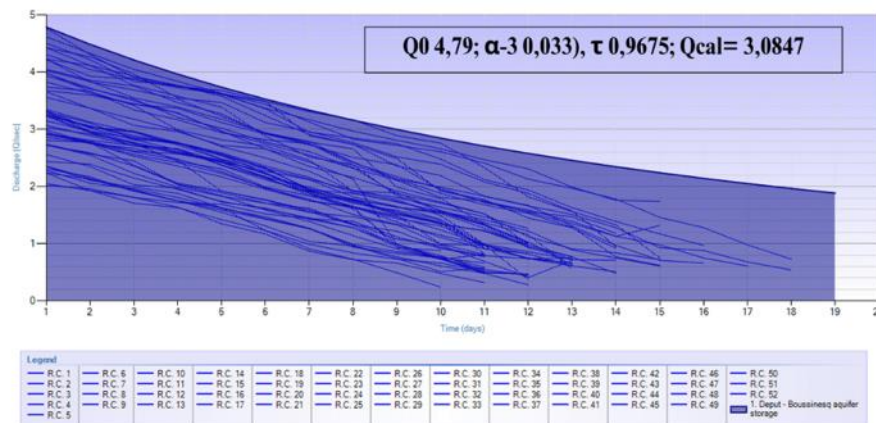
Fig. 2. MRC using the Dupuit-Boussinesq aquifer storage model for the Wae Batu Merah Watershed.
